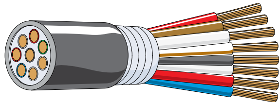
8 Conductor
