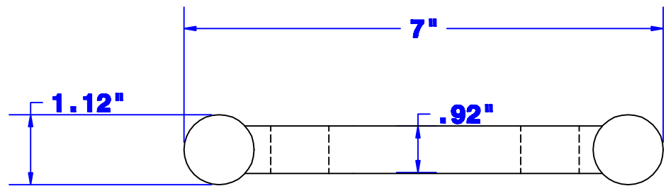
End View
