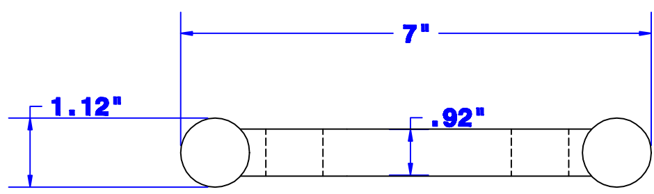
End View
