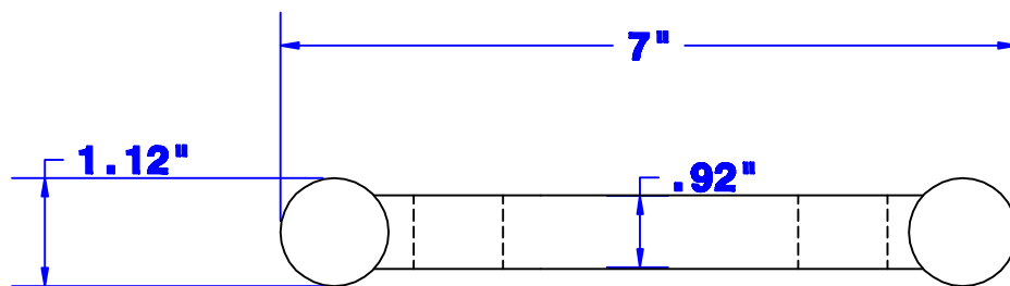
End View
